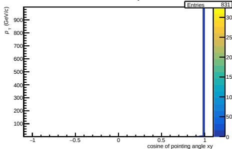
/hf-task-lc/Data/hCPAxyVsPt OLD
