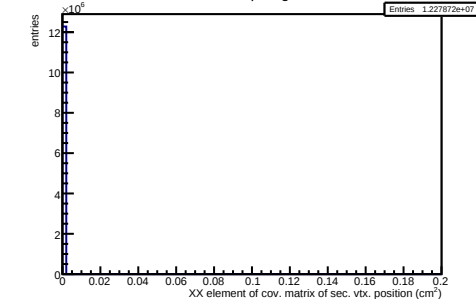
/hf-candidate-creator-3prong/hCovSVXX OLD
