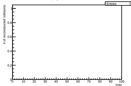
/hf-candidate-creator-3prong-expressions/hRecCollisionsCentMc NEW
