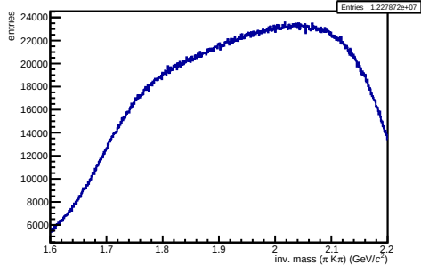
/hf-candidate-creator-3prong/hMass3PiKPi OLD
