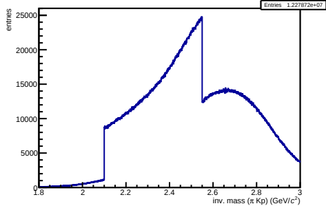
/hf-candidate-creator-3prong/hMass3PiKp OLD
