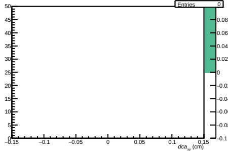
/propagation-service/hDCAxyVsPtRec OLD
