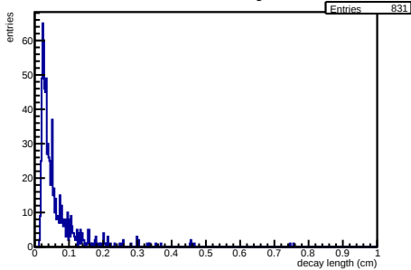
/hf-task-lc/Data/hDecLength OLD
