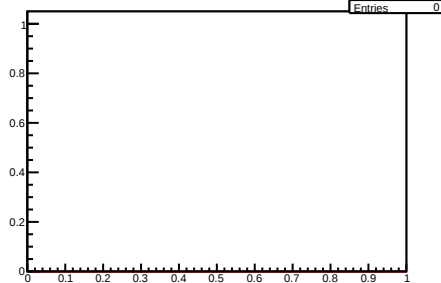
/eventselection-run3/luminosity/hCounterTVXZDafterBCcuts DIFF bins=0/3 max=0 min=0
