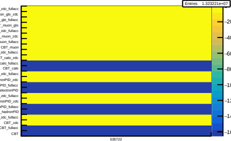
/eventselection-run3/luminosity/hLumiTCEafterBCutsRCT NEW
