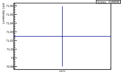
/eventselection-run3/luminosity/hLumiTVX NEW
