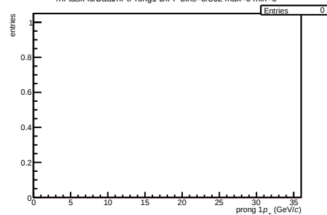
/hf-task-1c/Data/hPtProng1 DIFF bins=0/362 max=0 min=0
