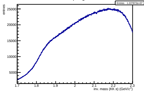
/hf-candidate-creator-3prong/hMass3KKPi OLD
