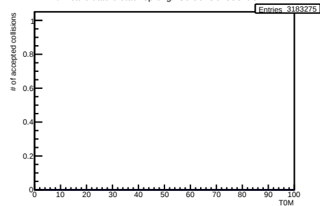
/hf-candidate-creator-3prong/hSelCollisionsCent OLD
