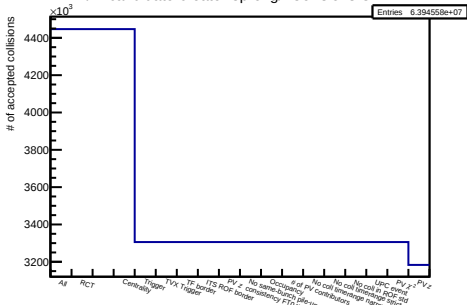
/hf-candidate-creator-3prong/hSelCollisionsCent OLD
