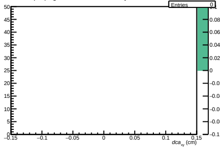
/propagation-service/hDCAxyVsPtMC NEW
