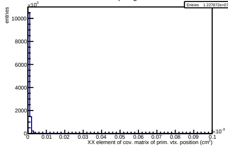
/hf-candidate-creator-3prong/hCovPVXX NEW
