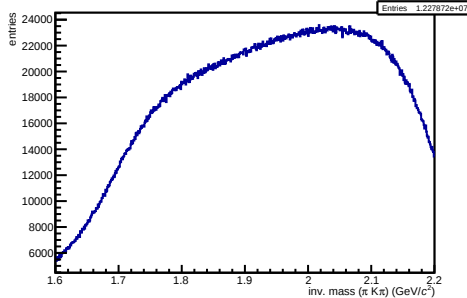
/hf-candidate-creator-3prong/hMass3PiKPi NEW
