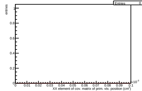
/hf-candidate-creator-3prong/hCovPVXX DIFF bins=0/102 max=0 min=0
