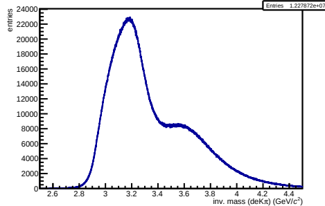
/hf-candidate-creator-3prong/hMass3DeKPi NEW
