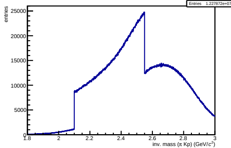
/hf-candidate-creator-3prong/hMass3PiKp NEW
