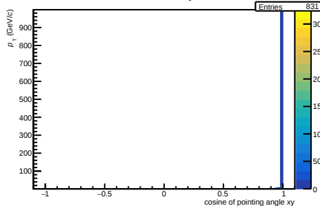
/hf-task-lc/Data/hCPAxyVsPt NEW
