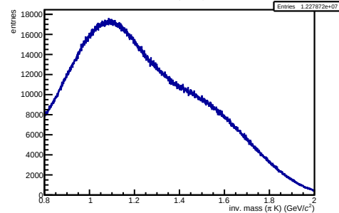
/hf-candidate-creator-3prong/hMass2PIK OLD
