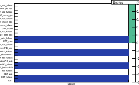
/eventselection-run3/luminosity/hLumiTCEafterBCutsRCT DIFF bins=0/78 max=0 min=0
