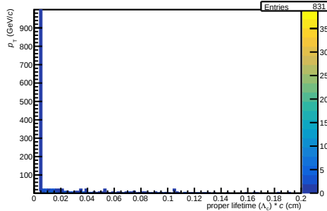
/hf-task-lc/Data/hCTVsPt NEW
