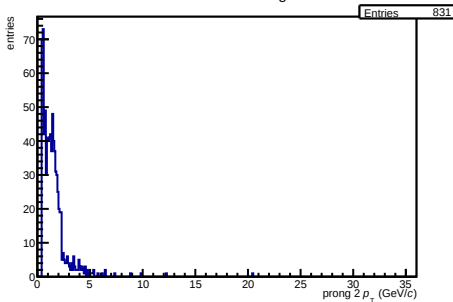
/hf-task-1c/Data/hd0Prong0 NEW
