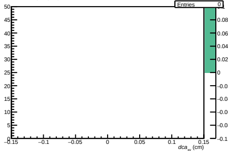
/propagation-service/hDCAzVsPtRec NEW
