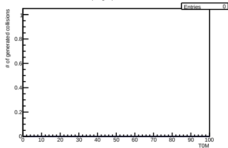
/hf-candidate-creator-3prong-expressions/hGenCollisionsCent OLD
