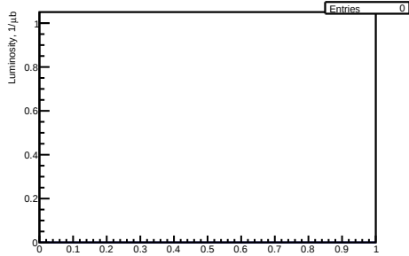
/eventselection-run3/luminosity/hLumiZNcafterBCuts OLD
