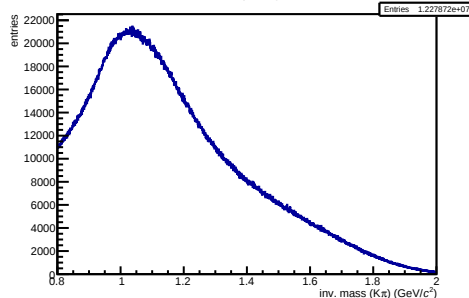
/hf-candidate-creator-3prong/hMass2KPi NEW
