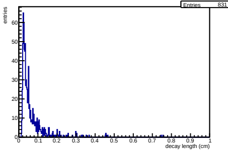
/hf-task-lc/Data/hDecLength NEW
