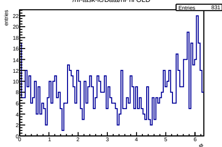
/hf-task-lc/Data/hPhi OLD
