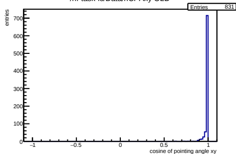
/hf-task-lc/Data/hCPAxy OLD
