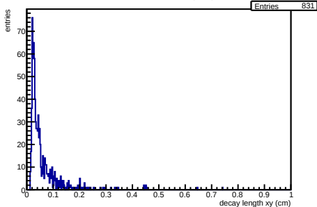
/hf-task-lc/Data/hDecLengthxy OLD
