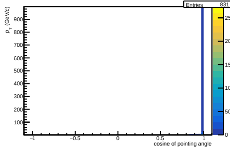
/hf-task-lc/Data/hCPAVsPt NEW
