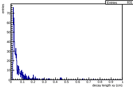
/hf-task-lc/Data/hDecLengthxy NEW
