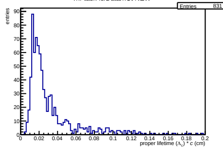
/hf-task-lc/Data/hCPA NEW
