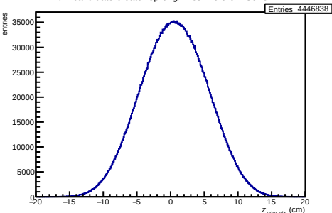
/hf-candidate-creator-3prong/hPosZBeforeEvSel OLD
