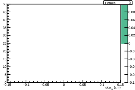
/propagation-service/hDCAzVsPtMC OLD
