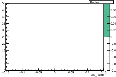
/propagation-service/hDCAxyVsPtRec NEW
