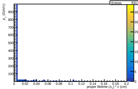
/hf-task-lc/Data/hCTVsPt OLD
