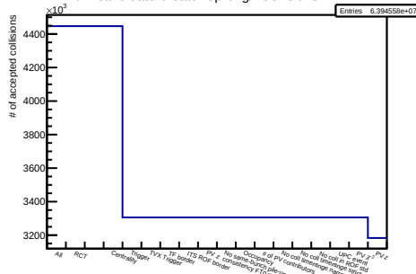
/hf-candidate-creator-3prong/hSelCollisionsCent NEW
