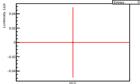
/eventselection-run3/luminosity/hLumiTVX DIFF bins=0/3 max=0 min=0
