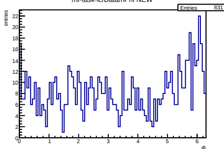
/hf-task-lc/Data/hPhi NEW
