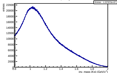
/hf-candidate-creator-3prong/hMass2KPi OLD
