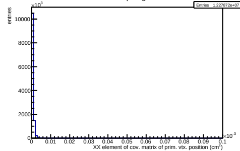
/hf-candidate-creator-3prong/hCovPVXX OLD
