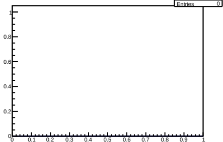
/eventselection-run3/luminosity/hCounterTVXZDafterBCcuts NEW
