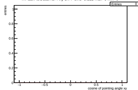
/hf-task-lc/Data/hCPAxy DIFF bins=0/112 max=0 min=0
