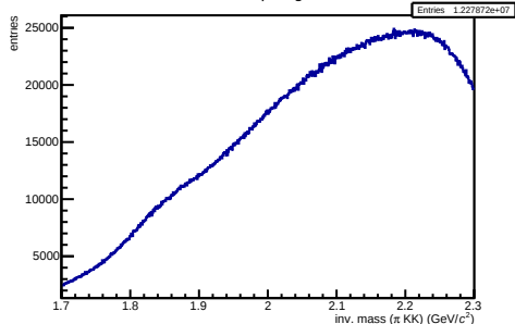
/hf-candidate-creator-3prong/hMass3PiKK OLD
