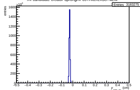
/hf-candidate-creator-3prong/hPosYAfterEvSel NEW
