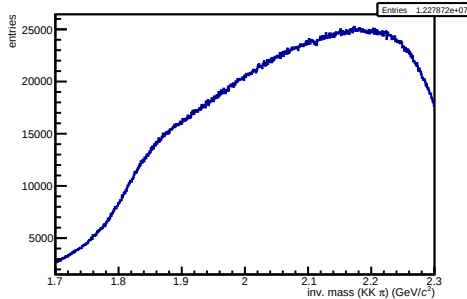
/hf-candidate-creator-3prong/hMass3KKPi NEW
