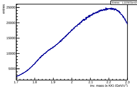
/hf-candidate-creator-3prong/hMass3PiKK NEW
