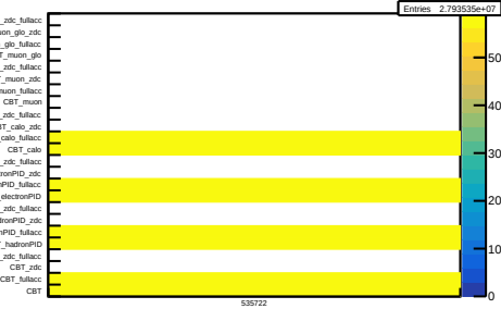
/eventselection-run3/luminosity/hLumiTVxafterBCutsRCT OLD
