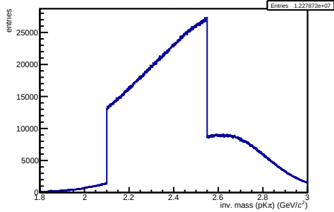
/hf-candidate-creator-3prong/hMass3PKPi OLD
