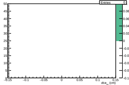
/propagation-service/hDCAzVsPtRec DIFF bins=0/34314 max=0 min=0
