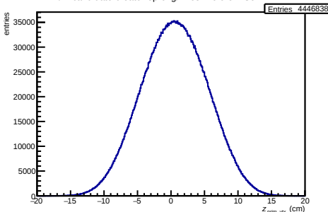
/hf-candidate-creator-3prong/hPosZBeforeEvSel NEW
