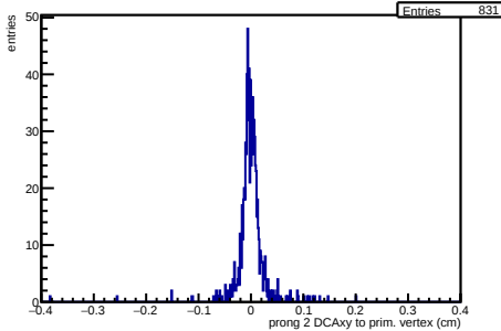
/hf-task-lc/Data/hd0Prong2 NEW
