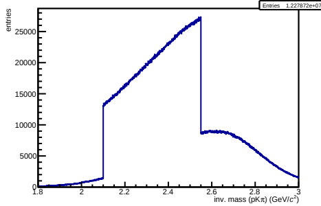
/hf-candidate-creator-3prong/hMass3PKPi NEW
