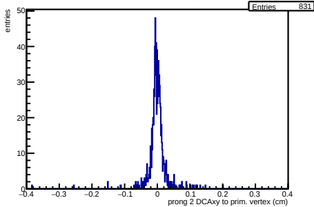
/hf-task-lc/Data/hd0Prong2 OLD
