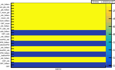
/eventselection-run3/luminosity/hLumiTCEafterBCutsRCT OLD
