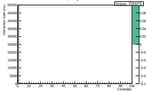
/hf-candidate-creator-3prong/hCollisionsCentIR OLD
