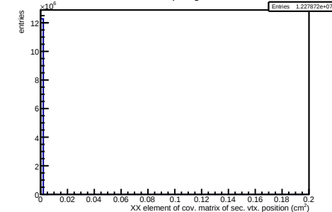
/hf-candidate-creator-3prong/hCovSVXX NEW
