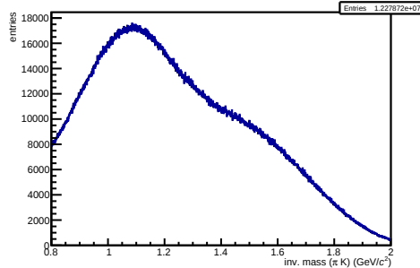
/hf-candidate-creator-3prong/hMass2PIK NEW
