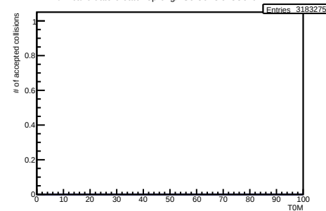
/hf-candidate-creator-3prong/hSelCollisionsCent NEW
