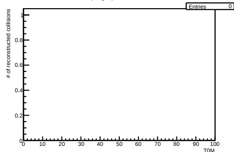
/hf-candidate-creator-3prong-expressions/hRecCollisionsCentMc OLD
