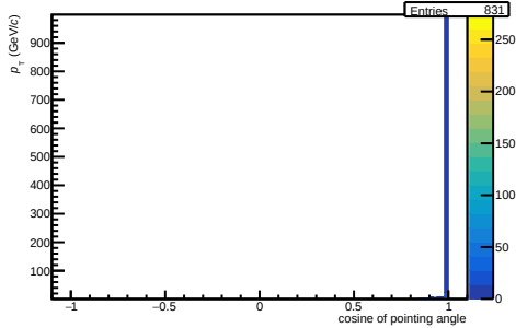
/hf-task-lc/Data/hCPAVsPt OLD
