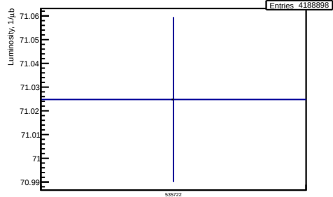
/eventselection-run3/luminosity/hLumiTVX OLD
