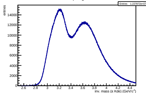
/hf-candidate-creator-3prong/hMass3PiKDe NEW
