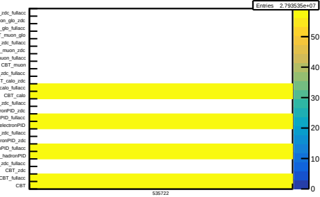
/eventselection-run3/luminosity/hLumiTVxafterBCutsRCT NEW
