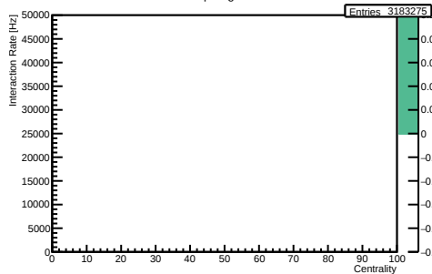
/hf-candidate-creator-3prong/hCollisionsCentIR NEW
